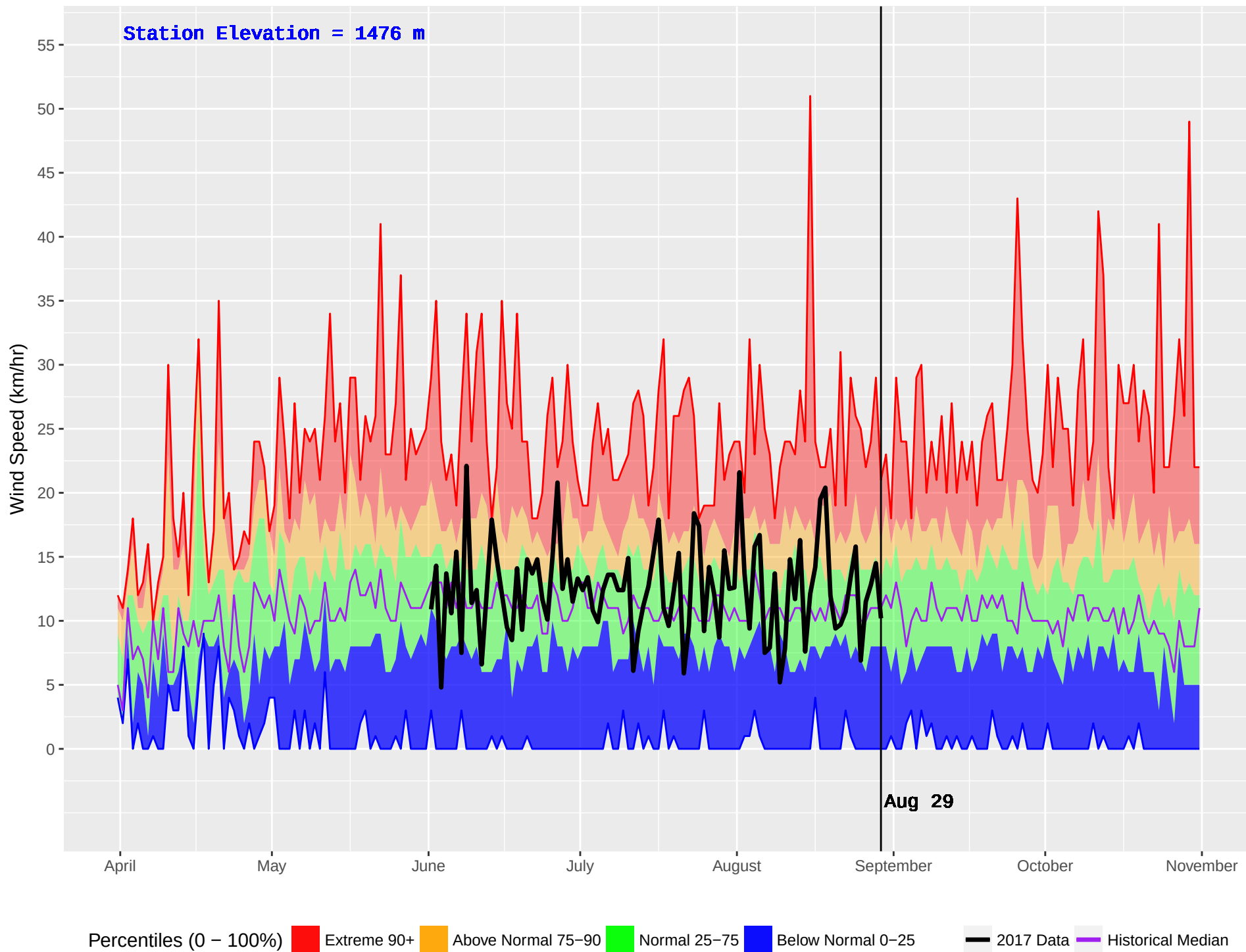
BRENDA MINES (283) : Historical (1977–2016) and Current (2017) Noon Wind Speed
